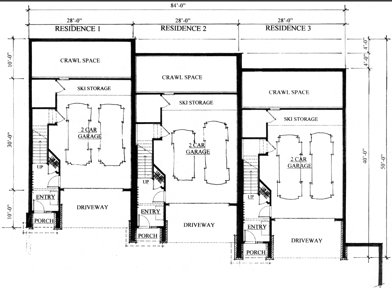
TOWN HOME UNITS 701 C, D & E - LOWER LEVEL
